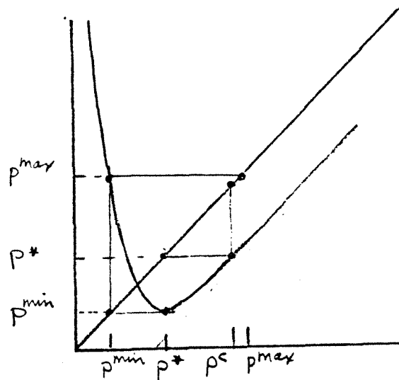
(b) The unstable case (chaos)
