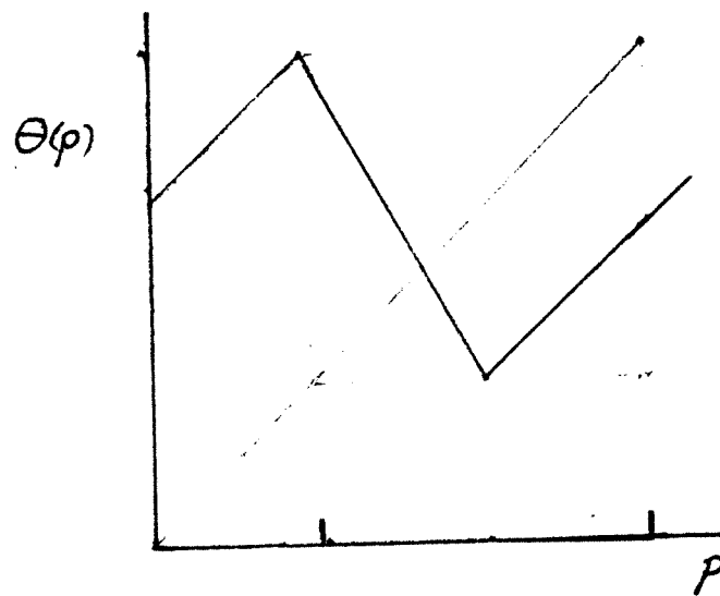
FIG 2.9. PIECEWISE LINEAR TATONNEMENT (all trajectories enter the trapping set)
