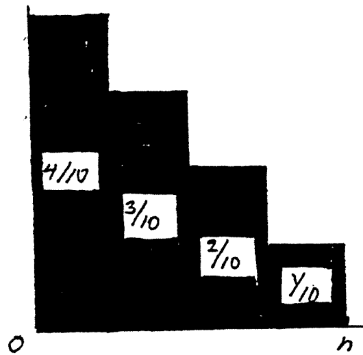
FIG 1.3. THE DENSITY FOR THE DYNAMICAL SYSTEM 1.9, n=4 .
