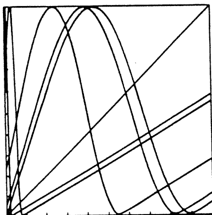
(a) Case I for several \mu
