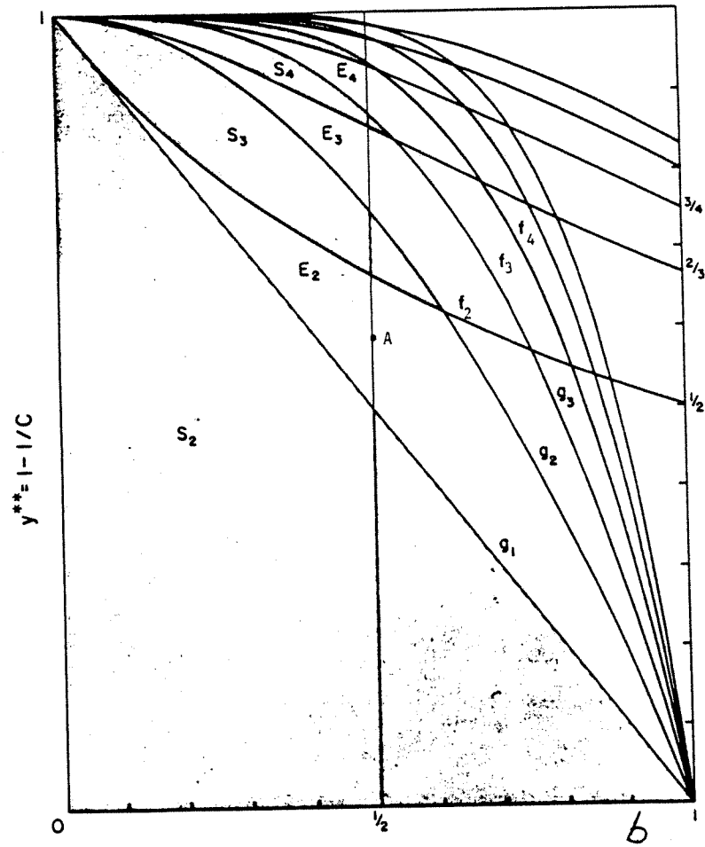
FIG 3.5. REGIONS OF STABLE AND ERGODIC BEHAVIOR (stable cycles appear in shaded regions; ergodic behavior appears in unshaded regions where \pi , S and b apply)
