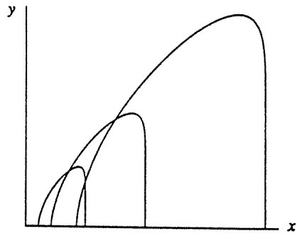
(a) Overlapping, almost smooth
