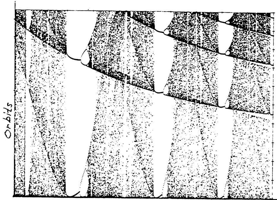
FIG 3.3. BIFURCATION DIAGRAM.
