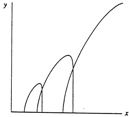
(b) Overlapping, kinked
