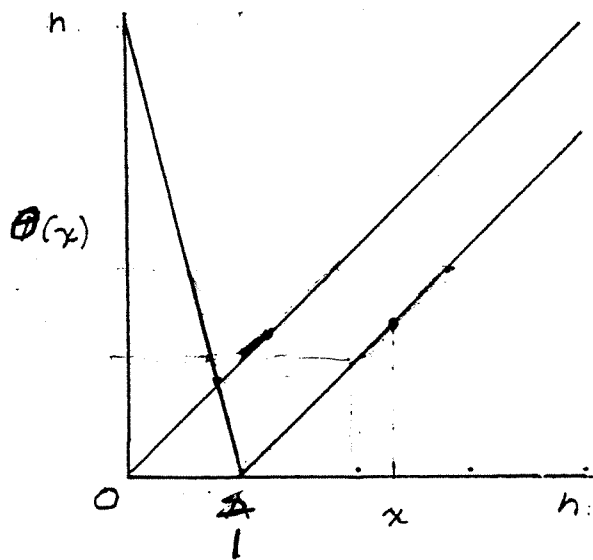
(a) the map for n=4
