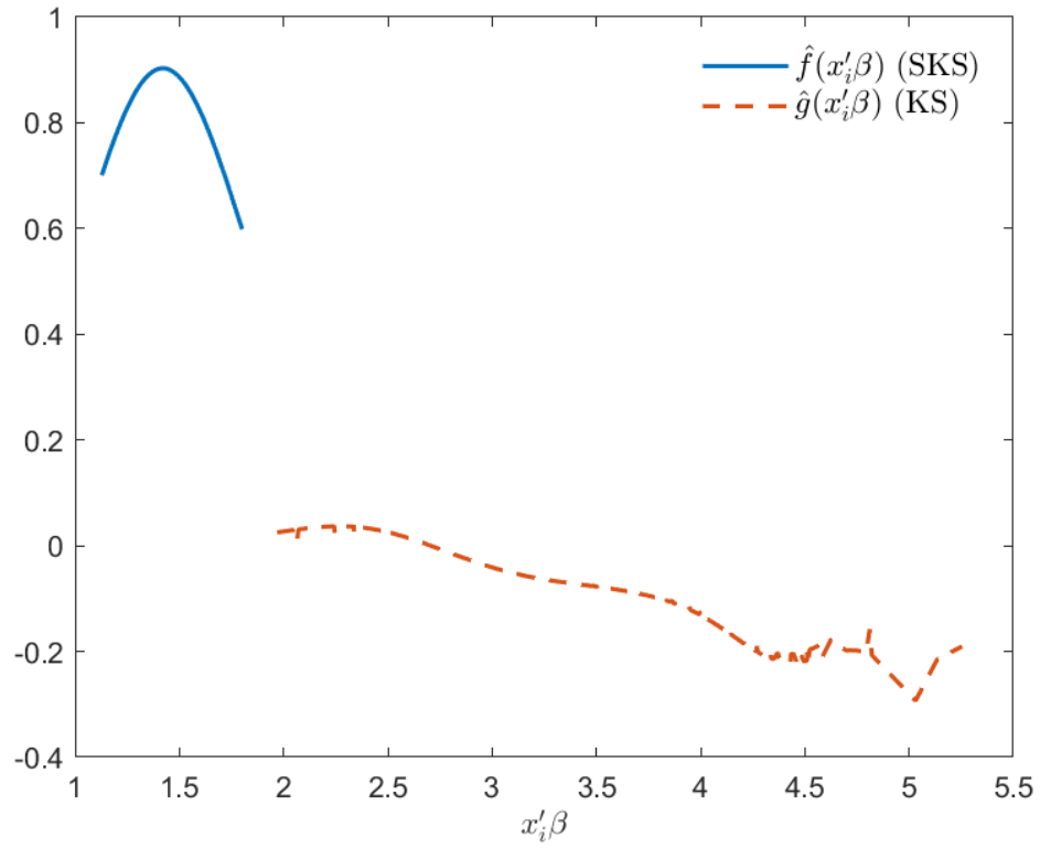
Figure 1: Plotting \hat{g}(x'_i\beta) and \hat{f}(x'_i\beta) over x'_i\beta .
